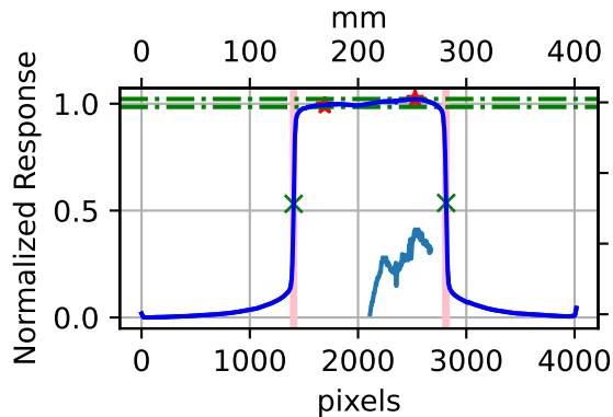
Horizontal Profile
