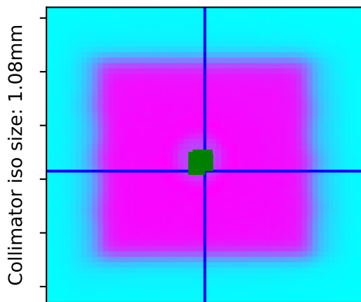
Collimator positions superimposed
