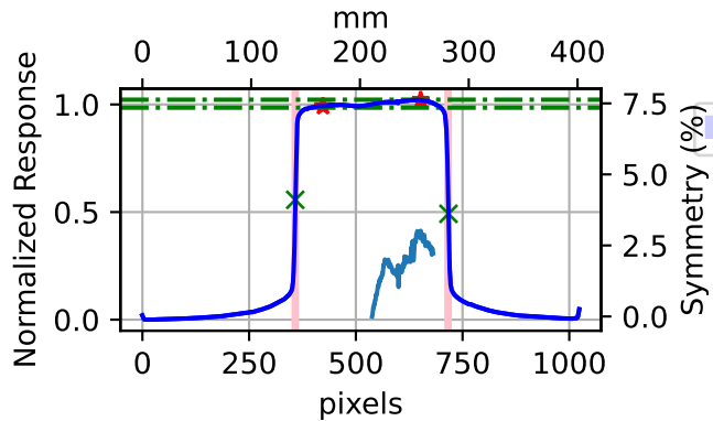
Horizontal Profile
